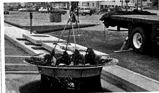
A CDS unit can be easily cleaned out in less than 30 minutes
