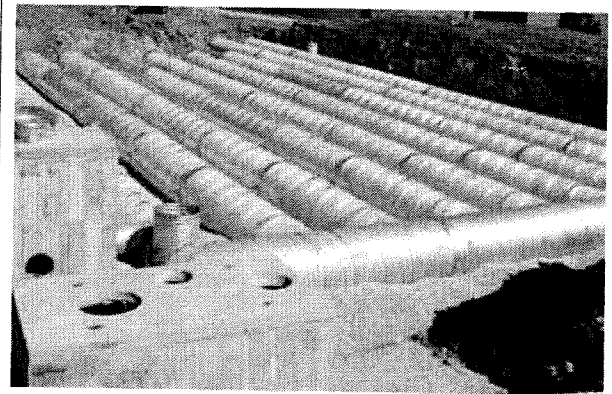
A Vortechs protects detention system from sediment build-up and reduces maintenance
